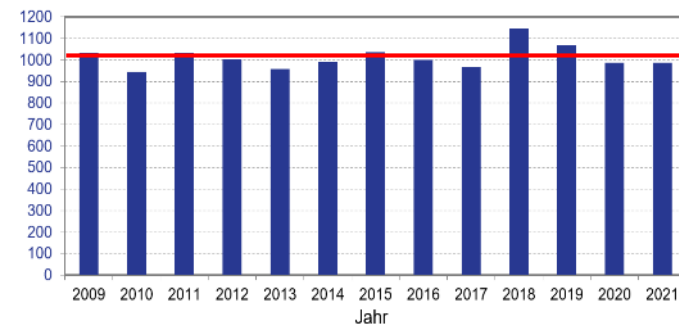
Ertrag in kWh/kWp
